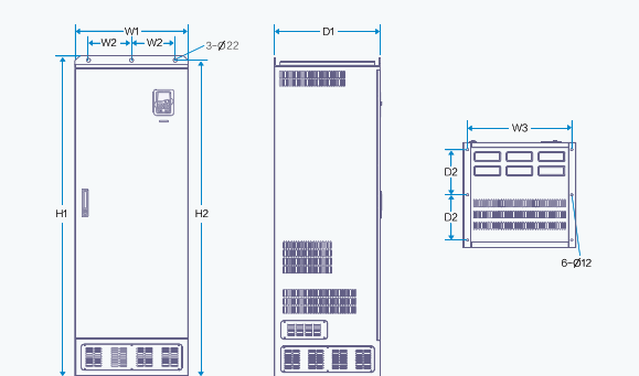
350-500kW Floor mounting Installation diagram
